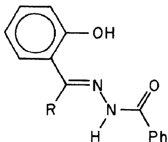
(20; H_2L' ; R = H, Me)
