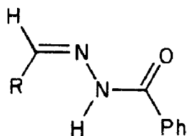
(18; HL; R = Ph, \overline{C_4H_3O} )
