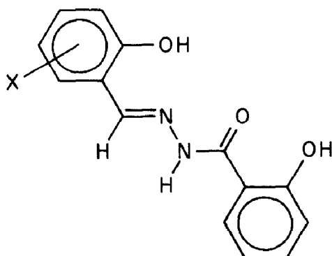
(22; H_2L' ; X = H, 5-Cl, 5-Br, 5-NO 2 , 3-OEt, 5-OMe, 3,5-Cl 2 , 5,6-benzo)
