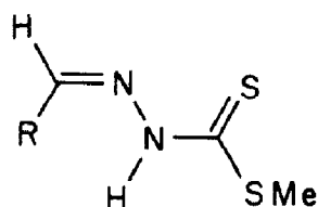
(19; HL; R = Ph, \overline{C_4H_3O} )
